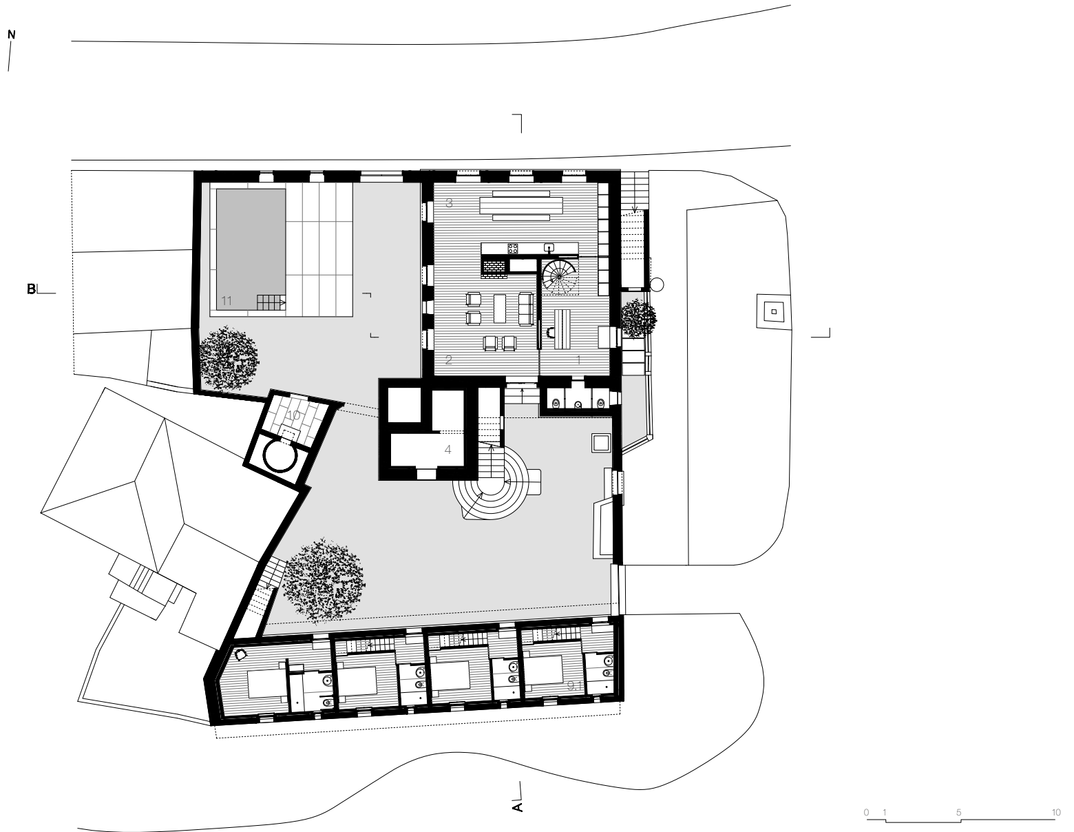
1. RECEPTION 2. LIVING ROOM 3. KITCHEN | DINING ROOM 4. TECHNICAL AREA 5. READING ROOM 6. BALCONY 7. GUEST ROOM 8. SUITE 9.1 DUPLEX (BEDROOM) 9.2 DUPLEX (LIVING ROOM) 10. WOOD OVEN 11. SWIMMING POOL
