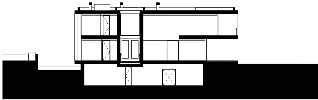
Section 1
