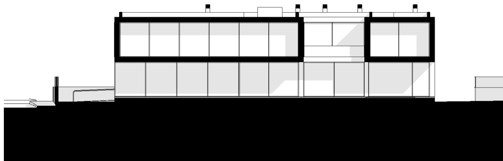
Section 3
