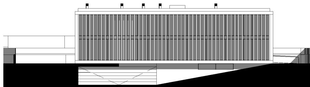
East Elevation
