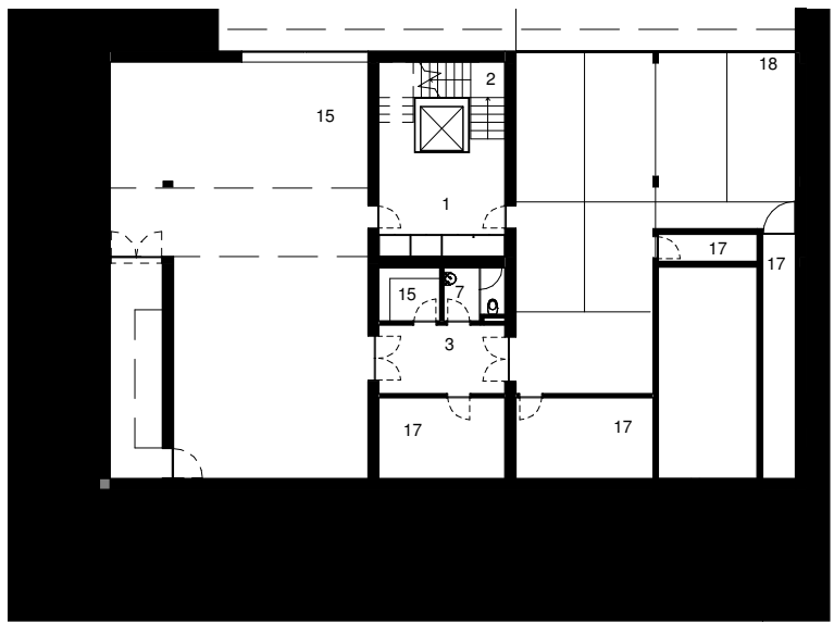
Basement Floor
