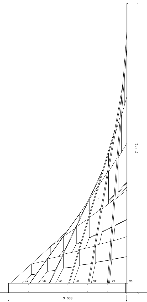
Northwest elevation
