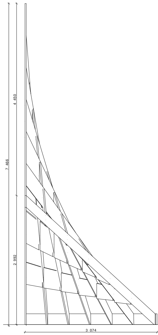
Southeast elevation
