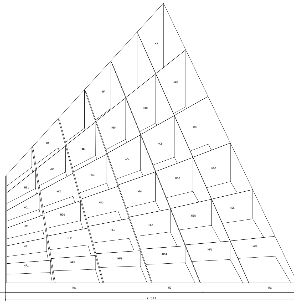
Southwest elevation
