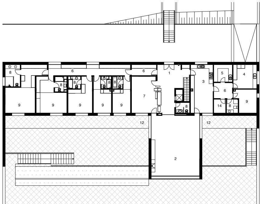
Planta do piso 1 First floor plan
