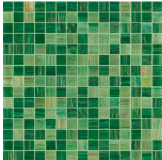
KILAUEA
