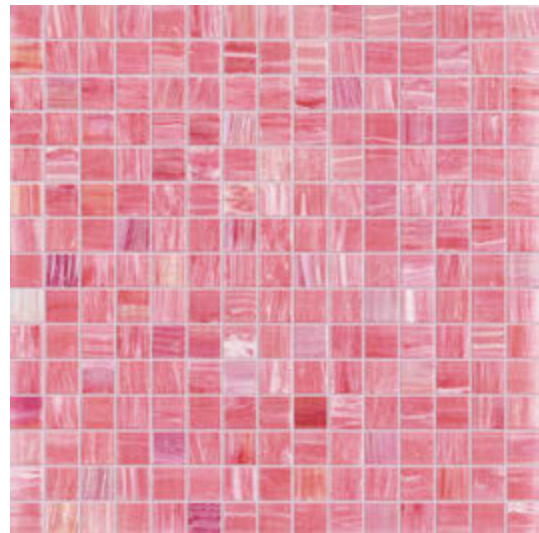
KRAKATOA
