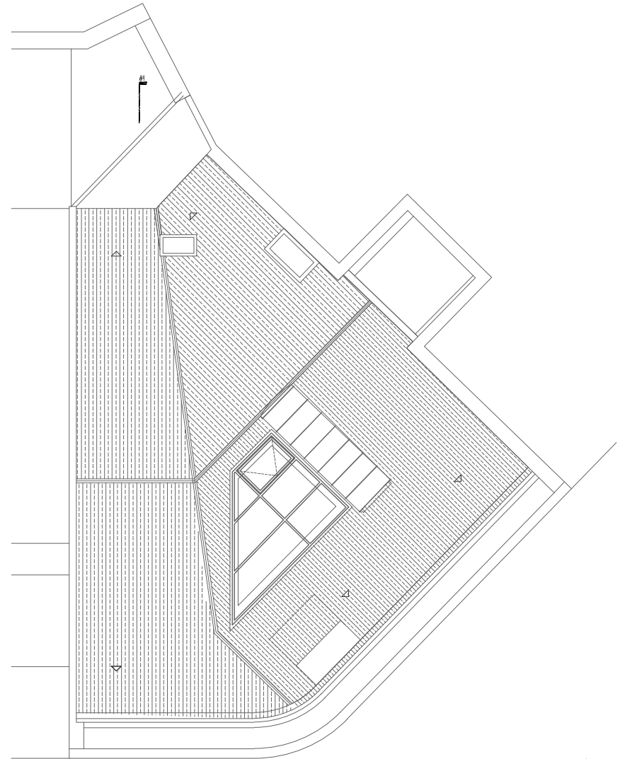
ROOF PLAN
