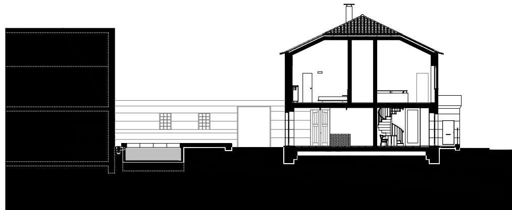
SECTION B
