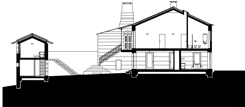
SECTION A
