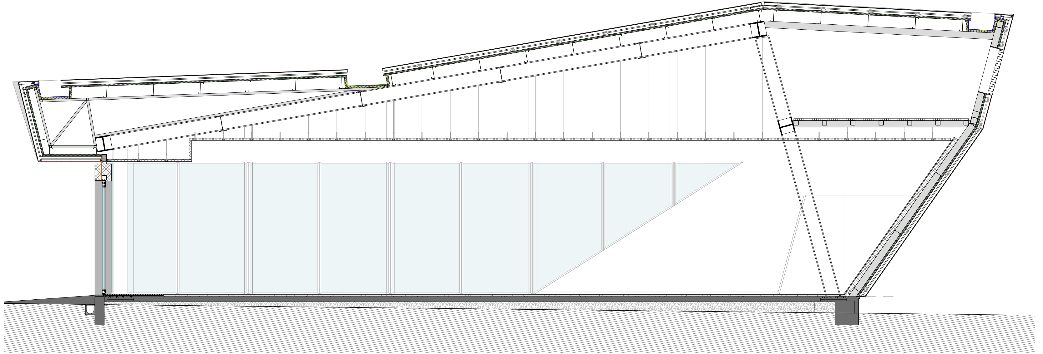
Section BB'
