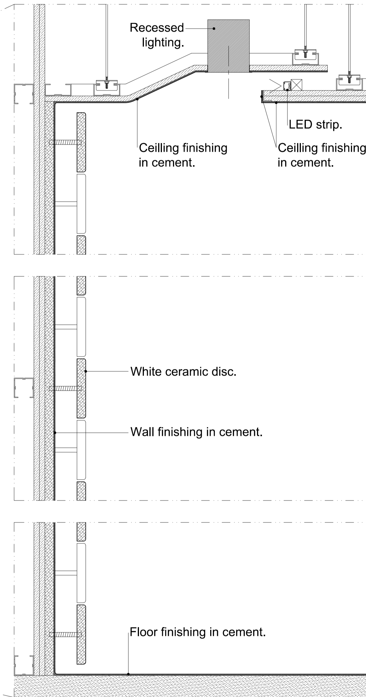
DETAIL (section)
