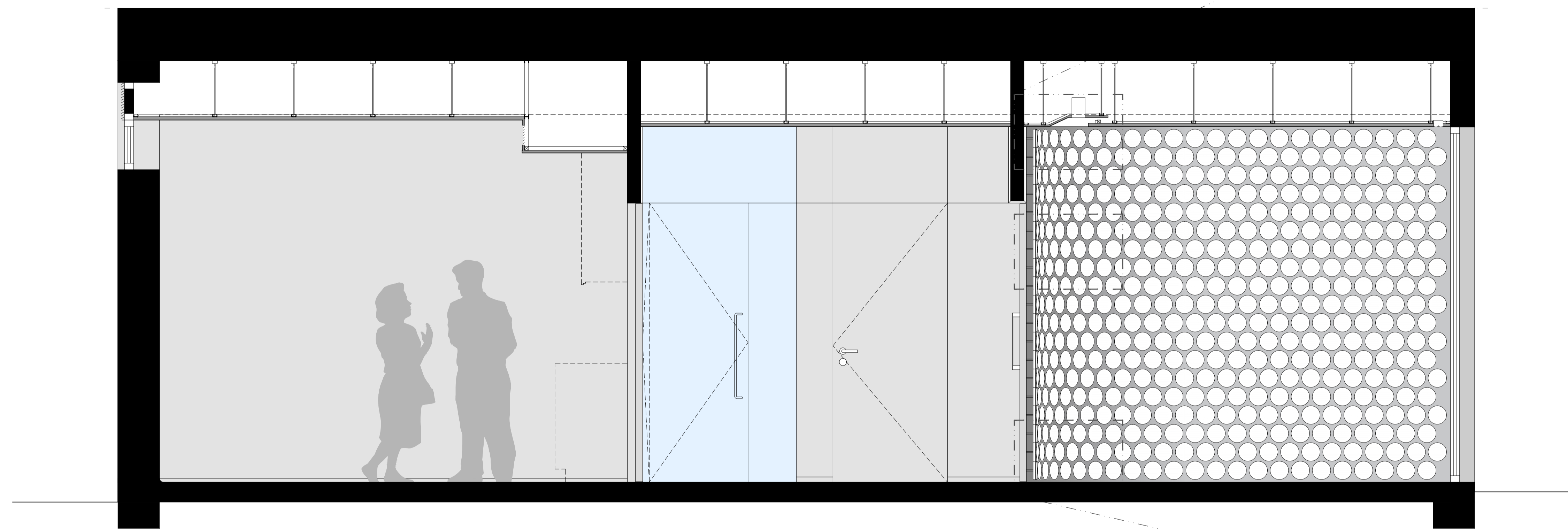
SECTION
