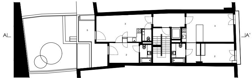
Planta piso 2 Second Floor Plan
