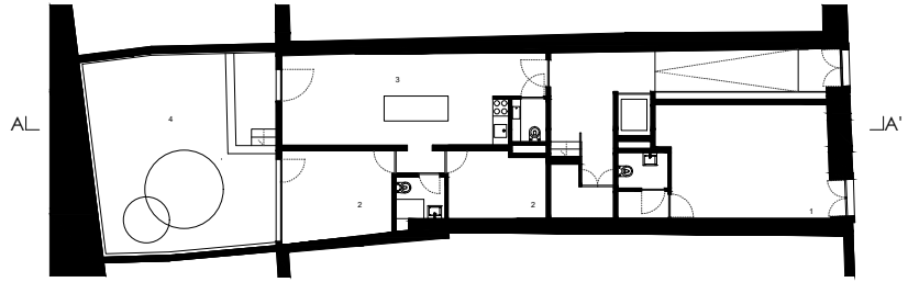
Planta piso 0 Ground Floor Plan
