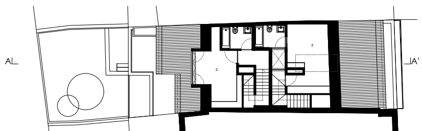
Planta piso 4 Fourth Floor Plan
