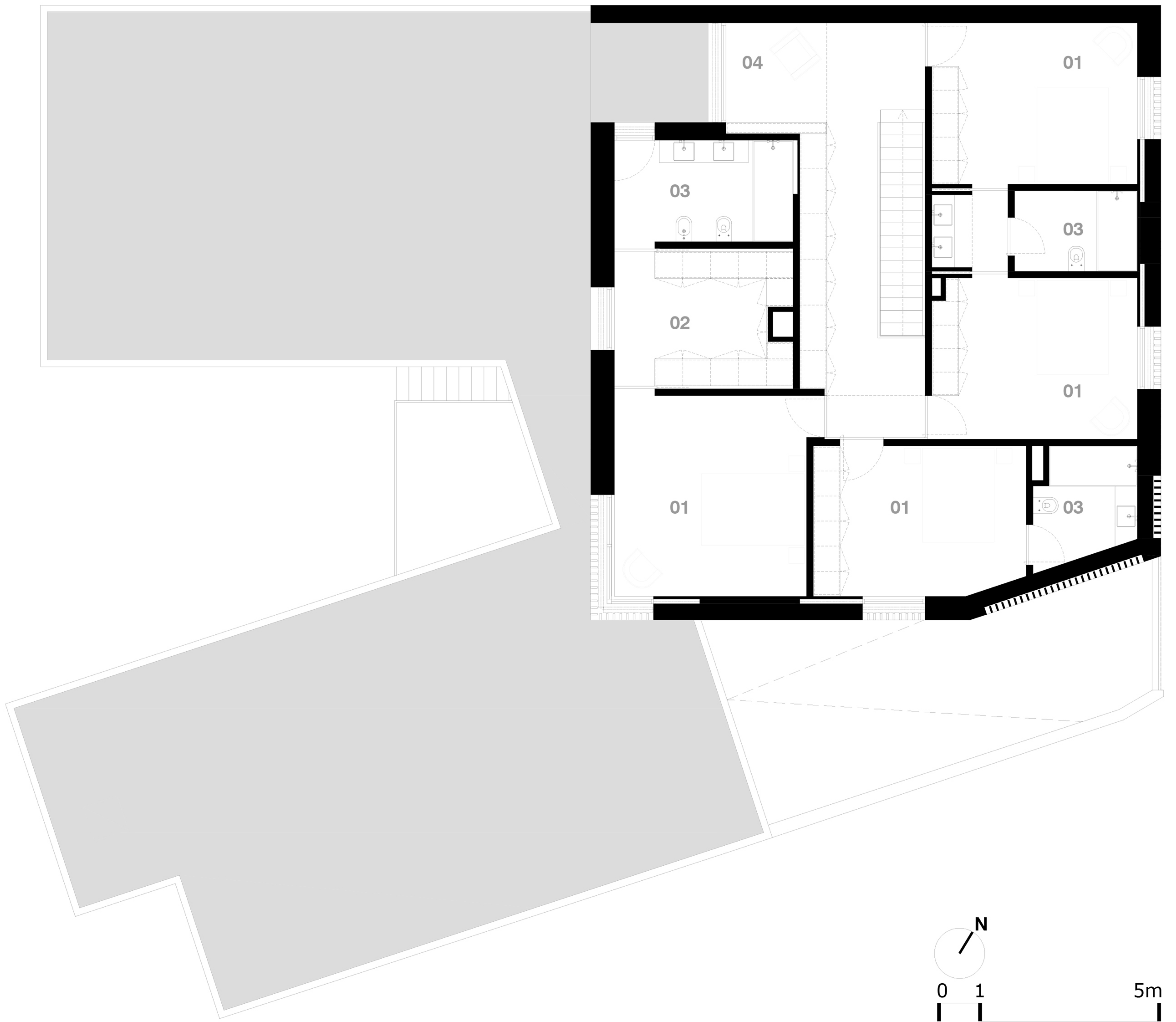
plan level 1
