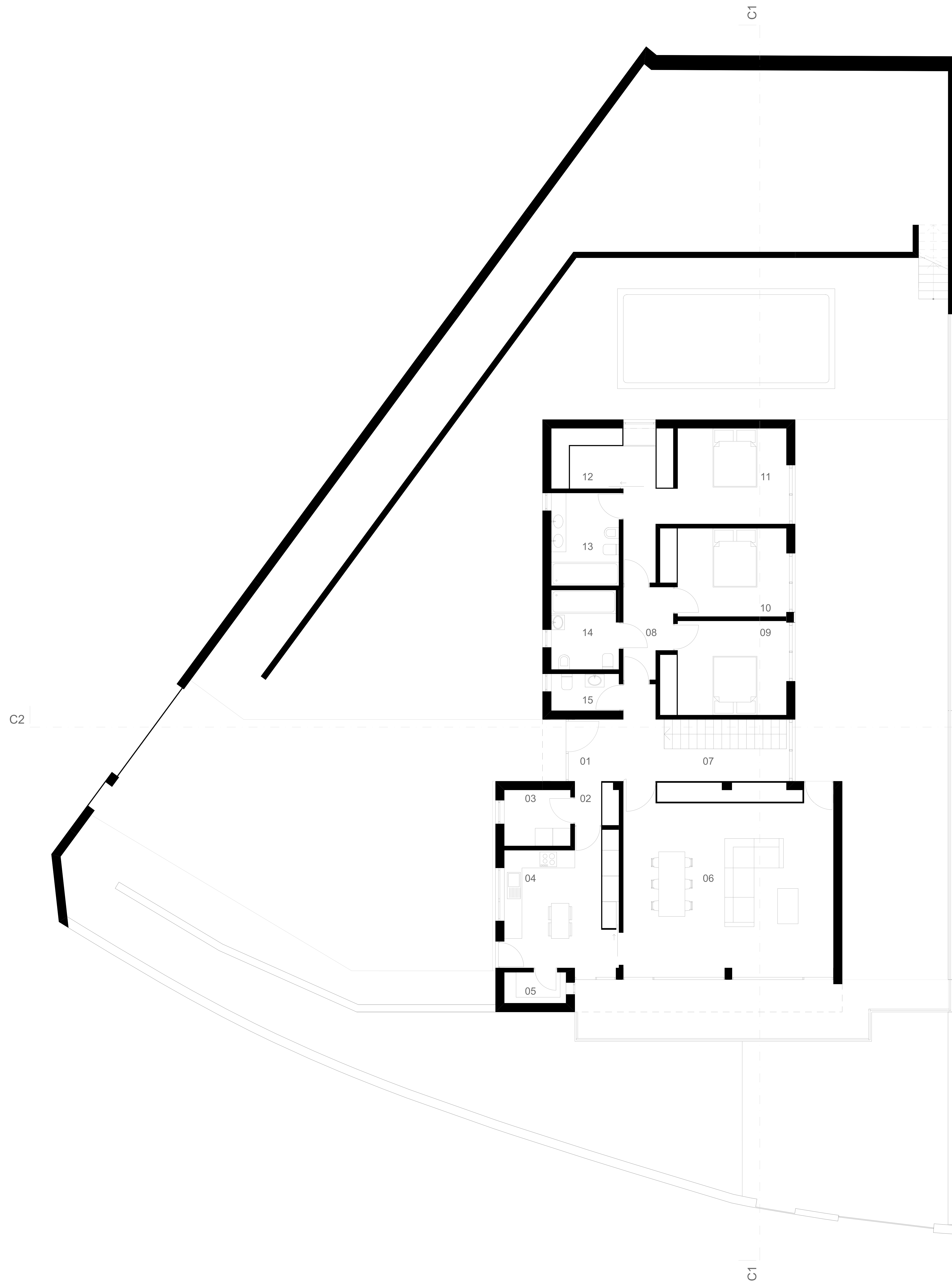
Ground floor plan
