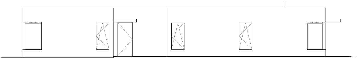
0 0.5 1 2 5 ELEVATION WEST
